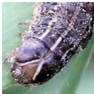
Figure 58. Fall armyworm (left) and corn earworm
